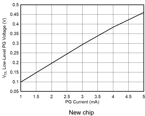
Figure 5-29. Low-Level PG Voltage vs Current
